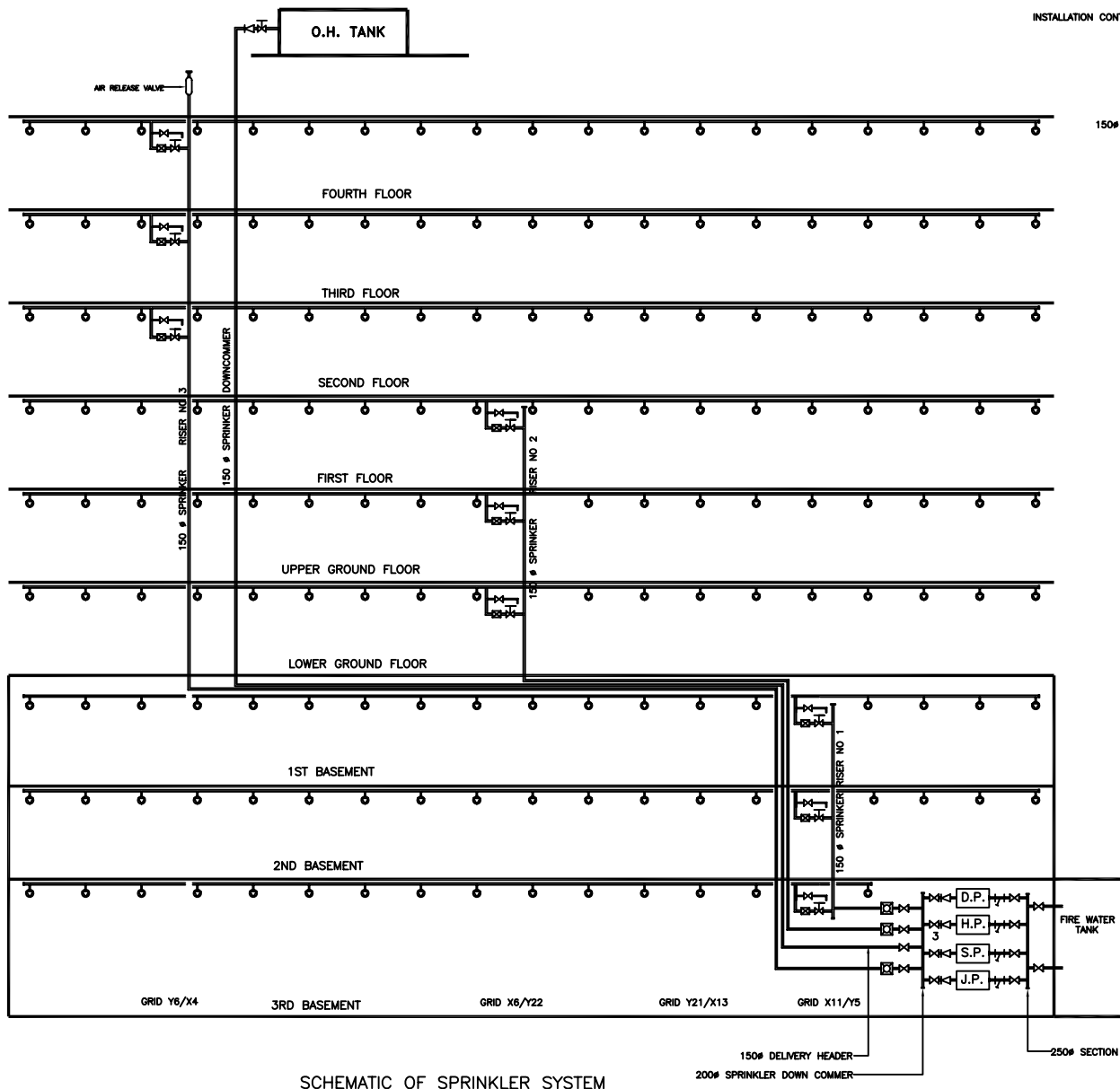
SCHEMATIC OF SPRINKLER SYSTEM
